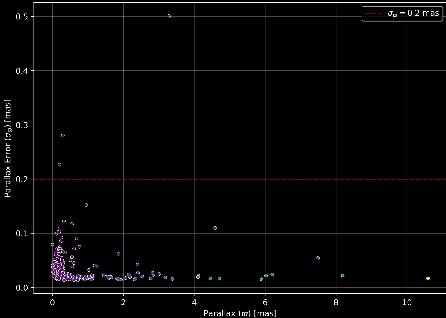
APOGEE DR17 Field: [Omegacen2] Parallax Quality (n= 456)
