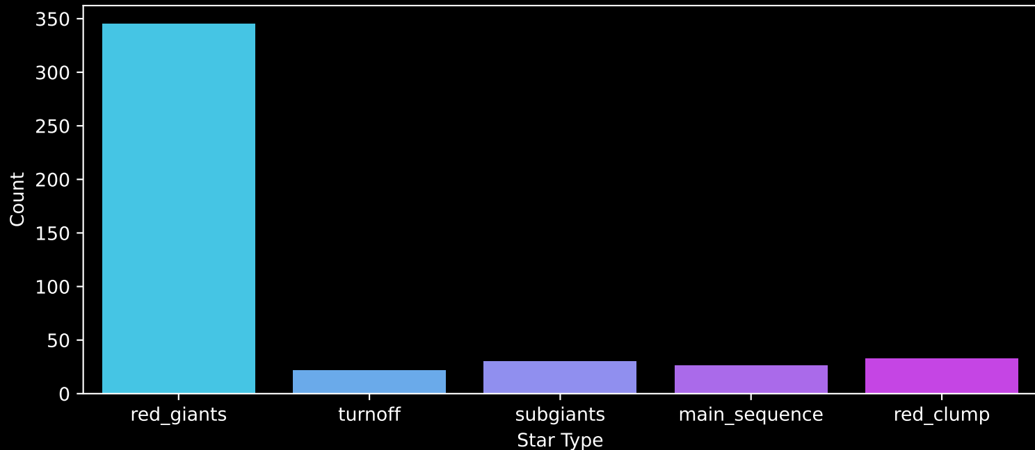
APOGEE DR17 Field: [Omegacen2] Count plot of Star Type
