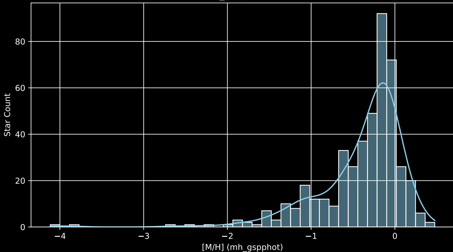
APOGEE DR17 Field: [Omgacen2 [M/H] (mh_gspphot) (n= 454)
