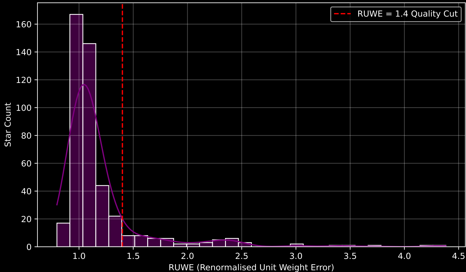
GAPOGEE DR17 Field [Omegacen2] RUWE Distribution (n= 452)
