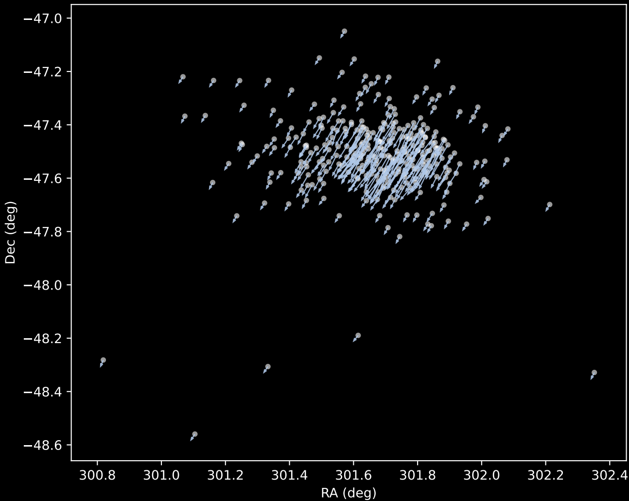
APOGEE DR17 Cluster 1 Proper Motion Vectors (n=314)
