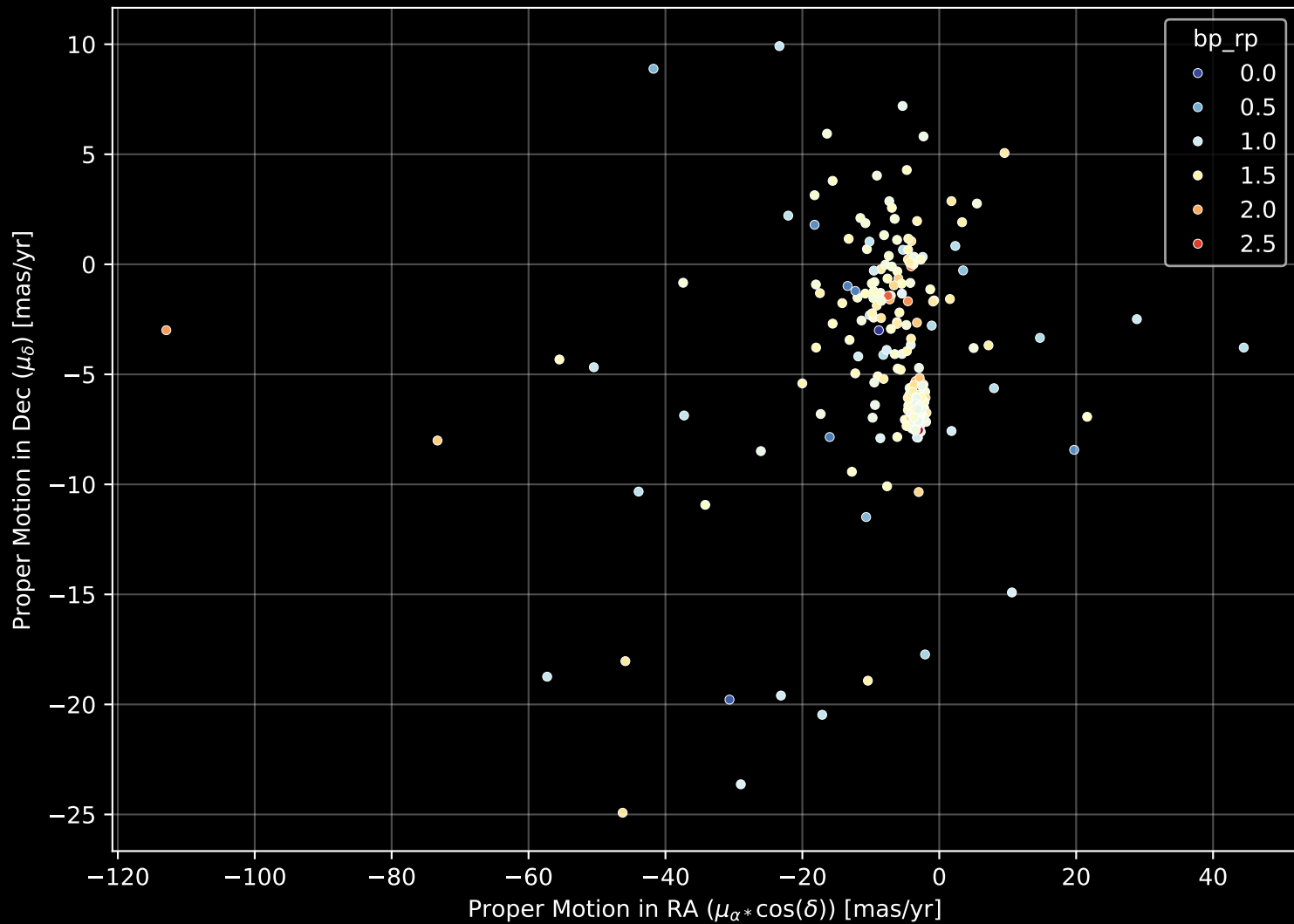
APOGEE DR17 Field: [Omegacen2] Proper Motion Diagram (n= 456)
