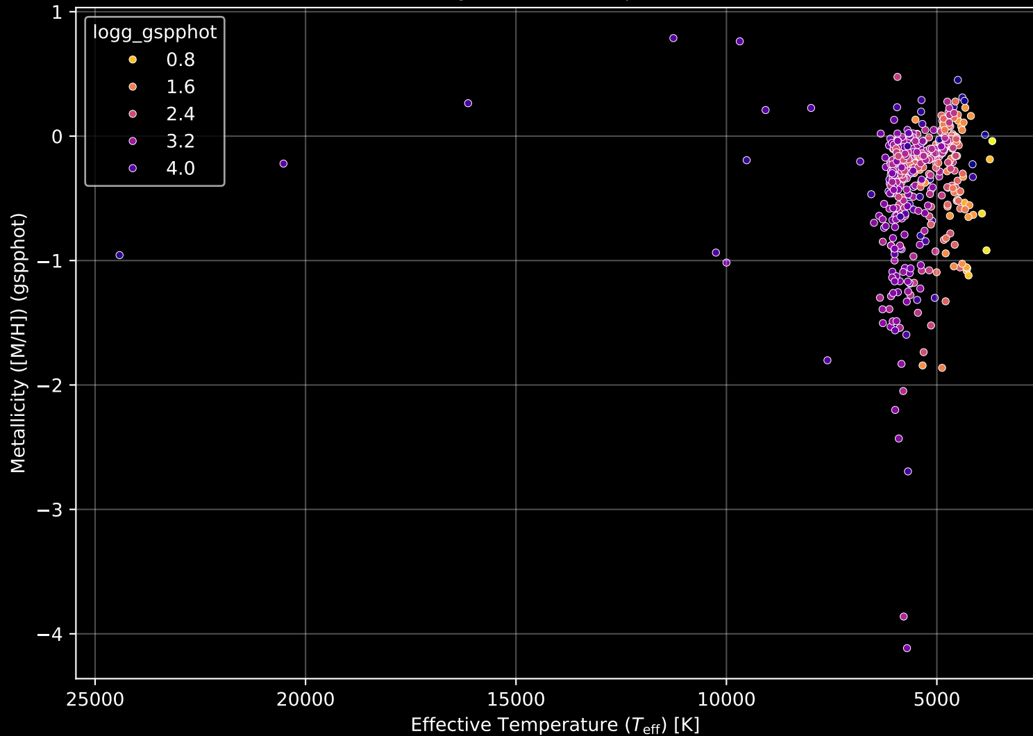
APOGEE DR17 Field: [Omegacen2] Stellar Population Parameters (n= 456)
